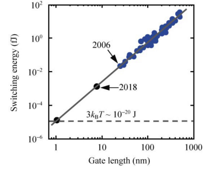
Figure 1.1: Energy cost of changing state for modern silicon transistors, as compared to a theoretical minimum for classical bits encoded in electron charge at room temperature ([CZH+06]). Figure reproduced from [Pop10, Figure 1(a)].
